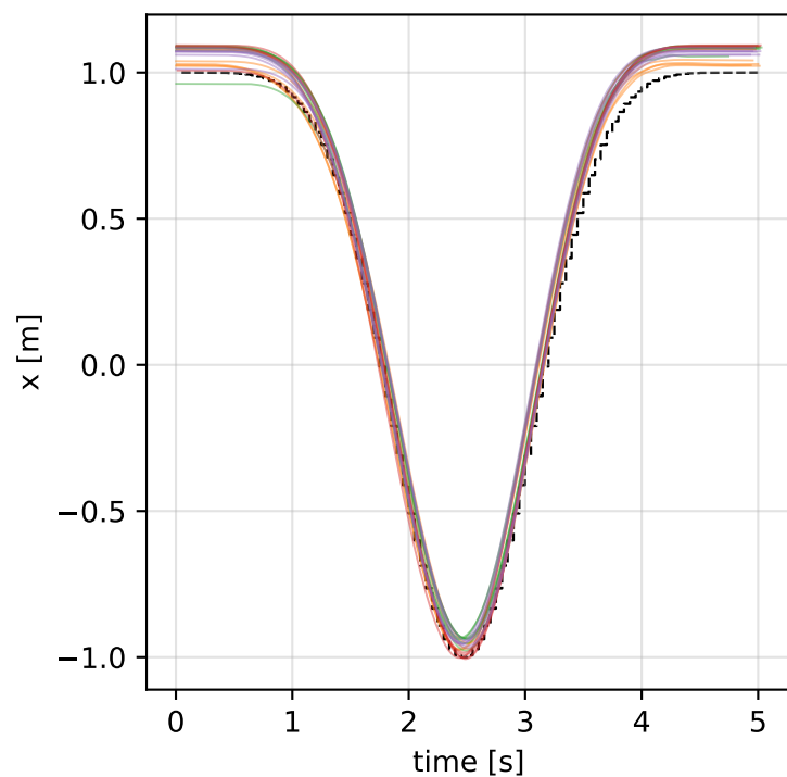
Gain MLP
